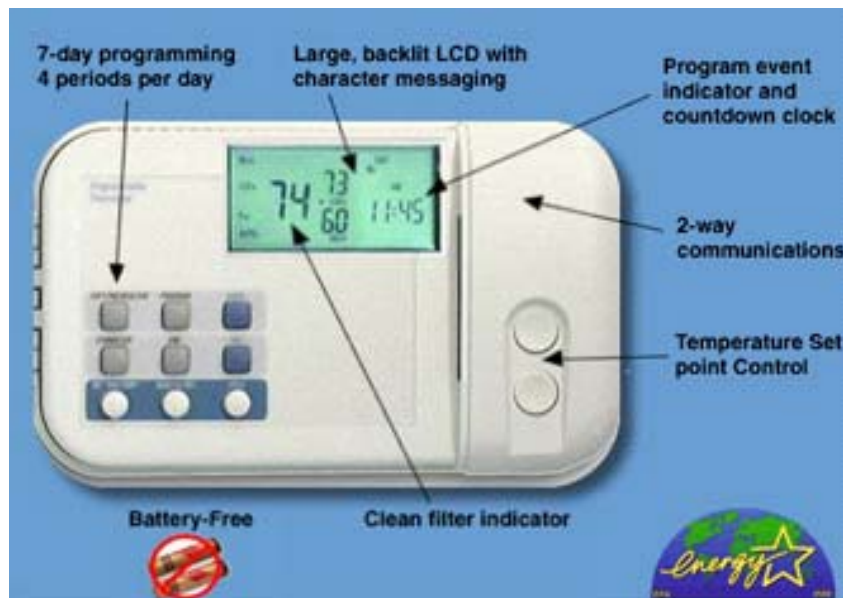
Figure 1. Carrier EMI Thermostat
