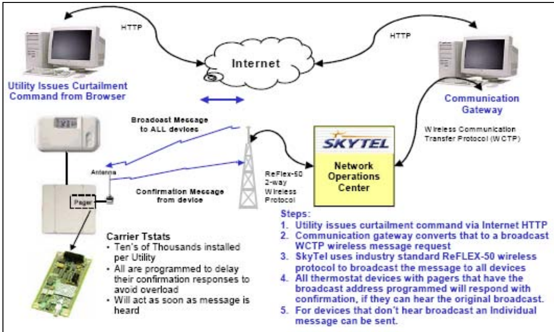
Figure 3. Broadcast Message Flow in the ComfortChoice System
