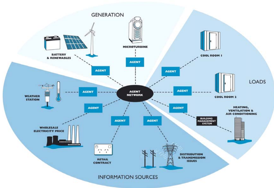
Figure 2. Demonstration GridAgent System at the CSIRO Energy Centre
