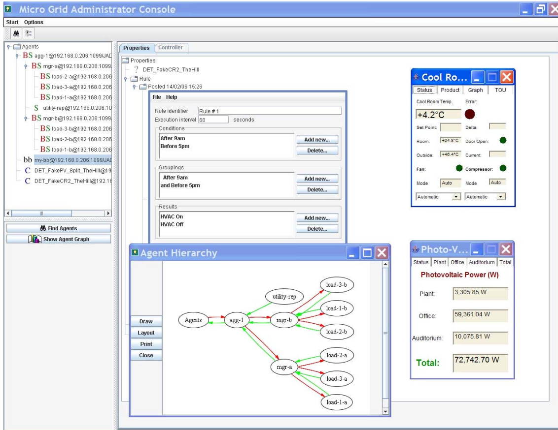
Figure 1. Web-based Management Console for the CSIRO GridAgents
