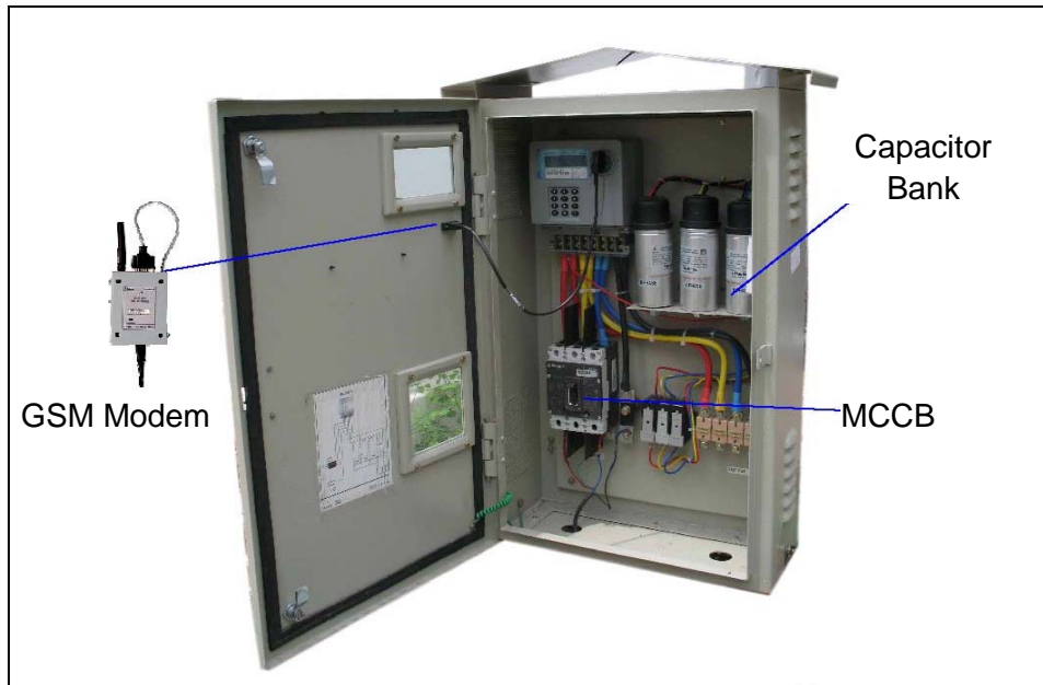
Figure 1. Components of the Lightchek System
