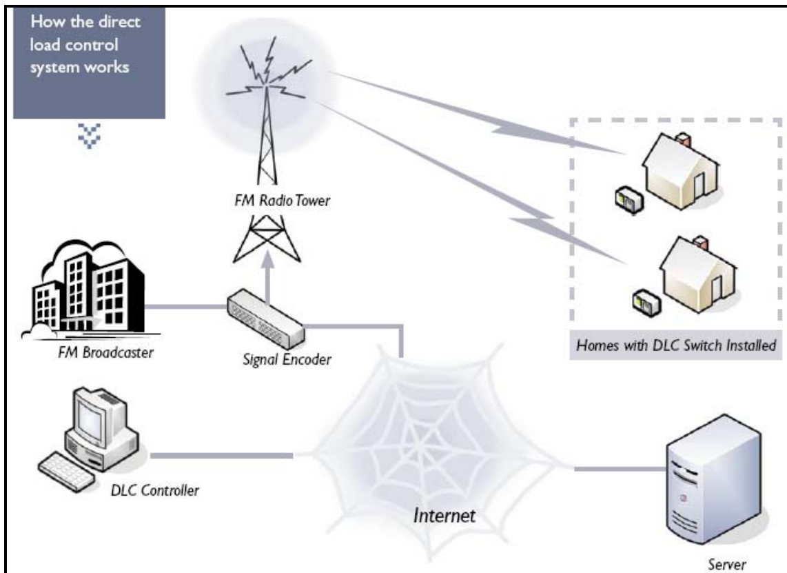
Figure 1. Components of the Saab Direct Load Control System
